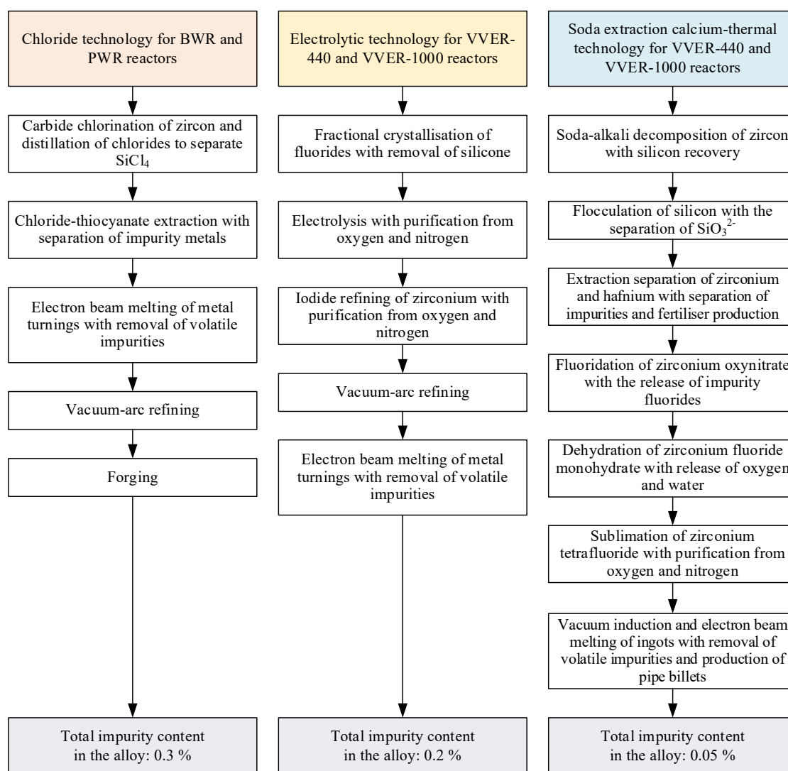
Figure 1 – Comparative analysis of different technological refining processes for the production of zirconium alloys for steam and water nuclear reactors
